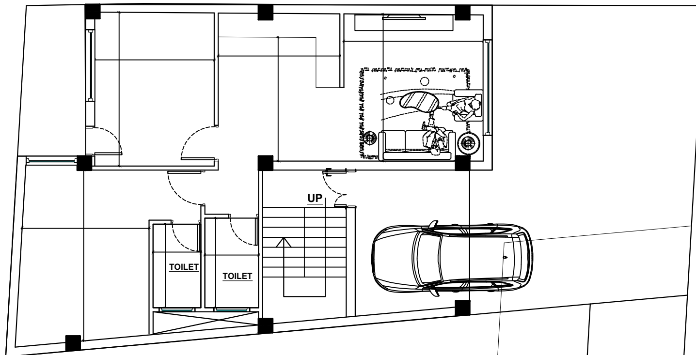
GROUND FLOOR AREA: 1010.26 SQ FT
